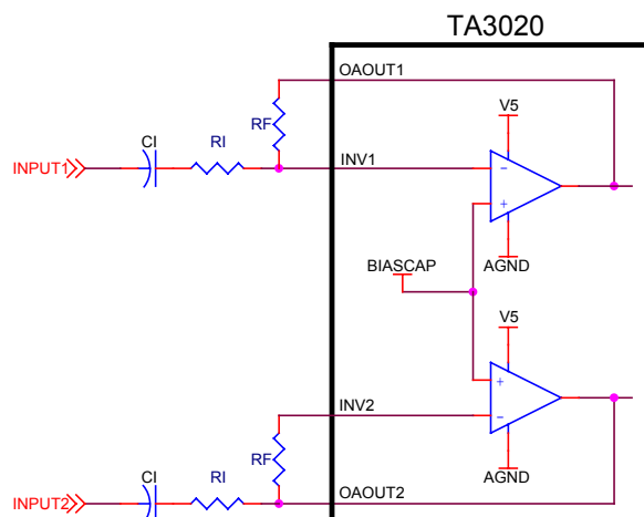
Figure 2: Input Stage
