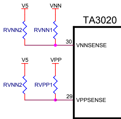
Figure 5: Over / Under voltage sense circuit
