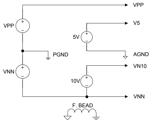
Figure 6: Proper Power Supply Connection
